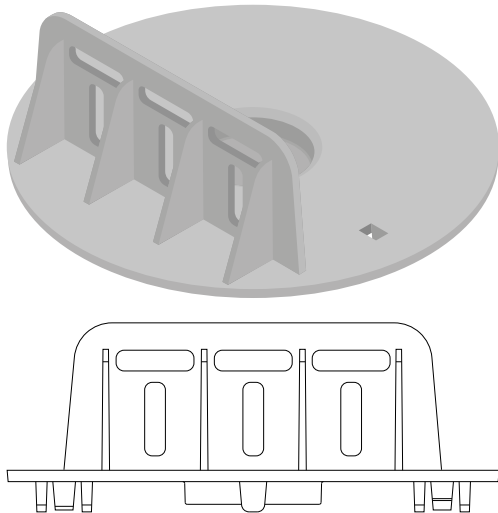
Cabezal Rastrel Madera Wood Batten Head
