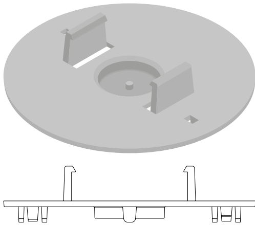
Cabezal Rastrel Aluminio Aluminum Batten Head
